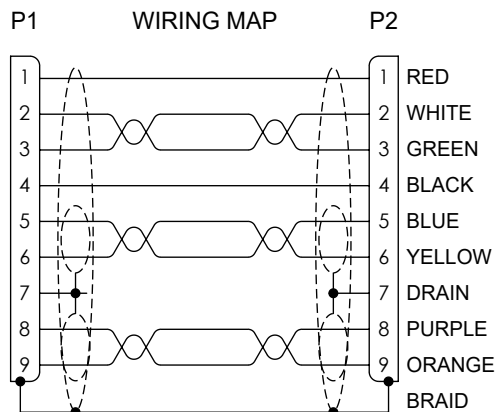
P1 USB 3.0 SERIES A MALE CONNECTOR
