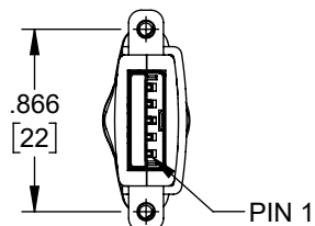
P1 USB 3.0 SERIES A MALE CONNECTOR
