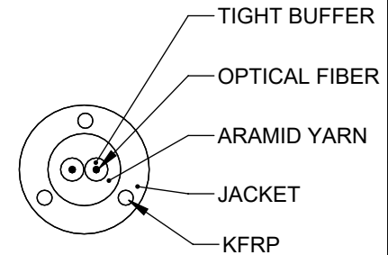
CABLE PROFILE VIEW
