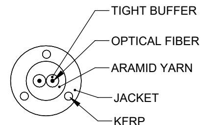
CABLE PROFILE VIEW
