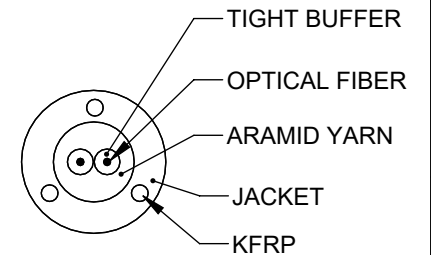
CABLE PROFILE VIEW
