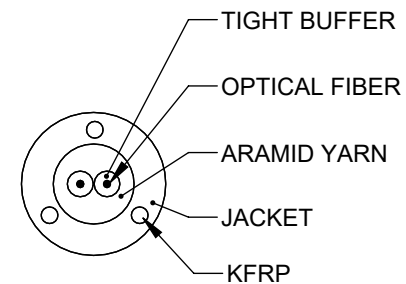
CABLE PROFILE VIEW
