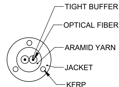
CABLE PROFILE VIEW
