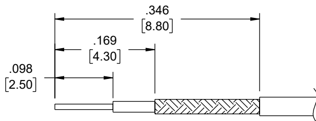
STRIPPING DIMENSIONS
