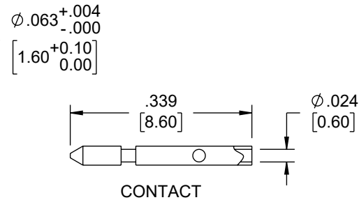
CONTACT
