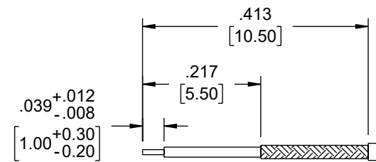
STRIPPING DIMENSIONS
