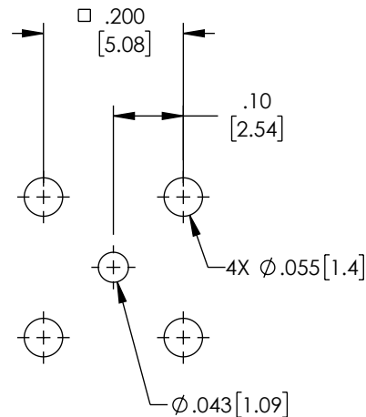
RECOMMENDED MTG HOLE PATTERN
